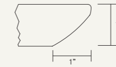
Edge Detail # 28 HPL laminate over a 1" MDF core counter balanced. The edge is cut back with a chamfer. The edge is clear finish as standard or can be stained.
